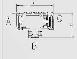
Forme B / Form B
